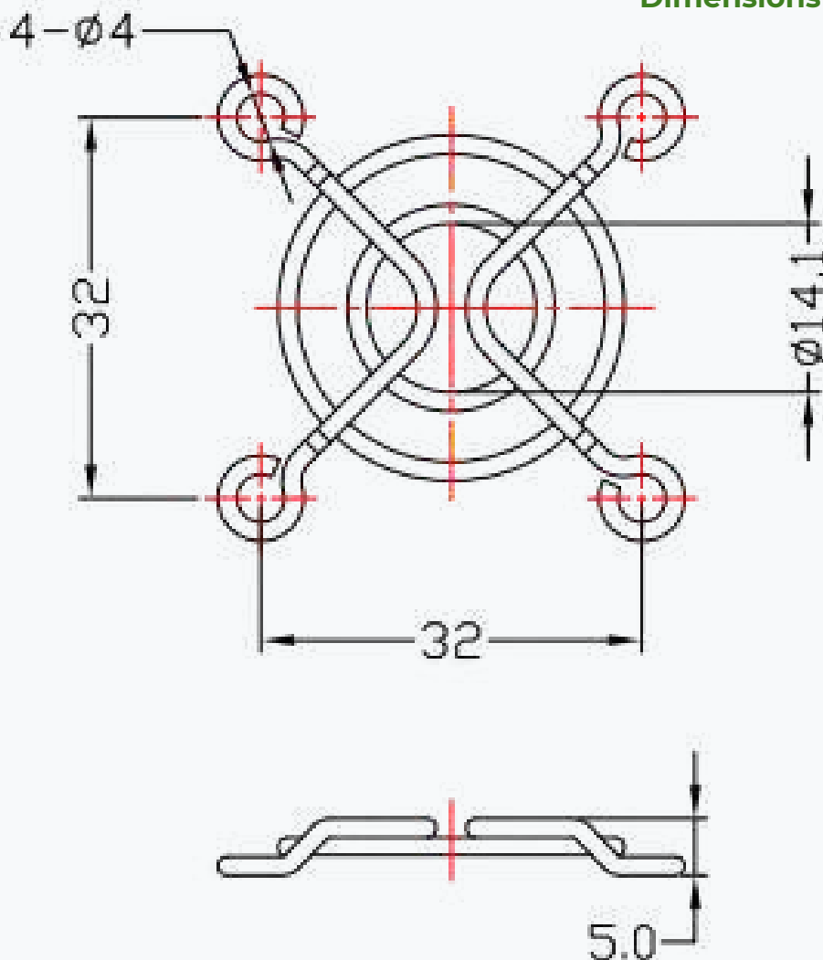
Dimensions (mm)
