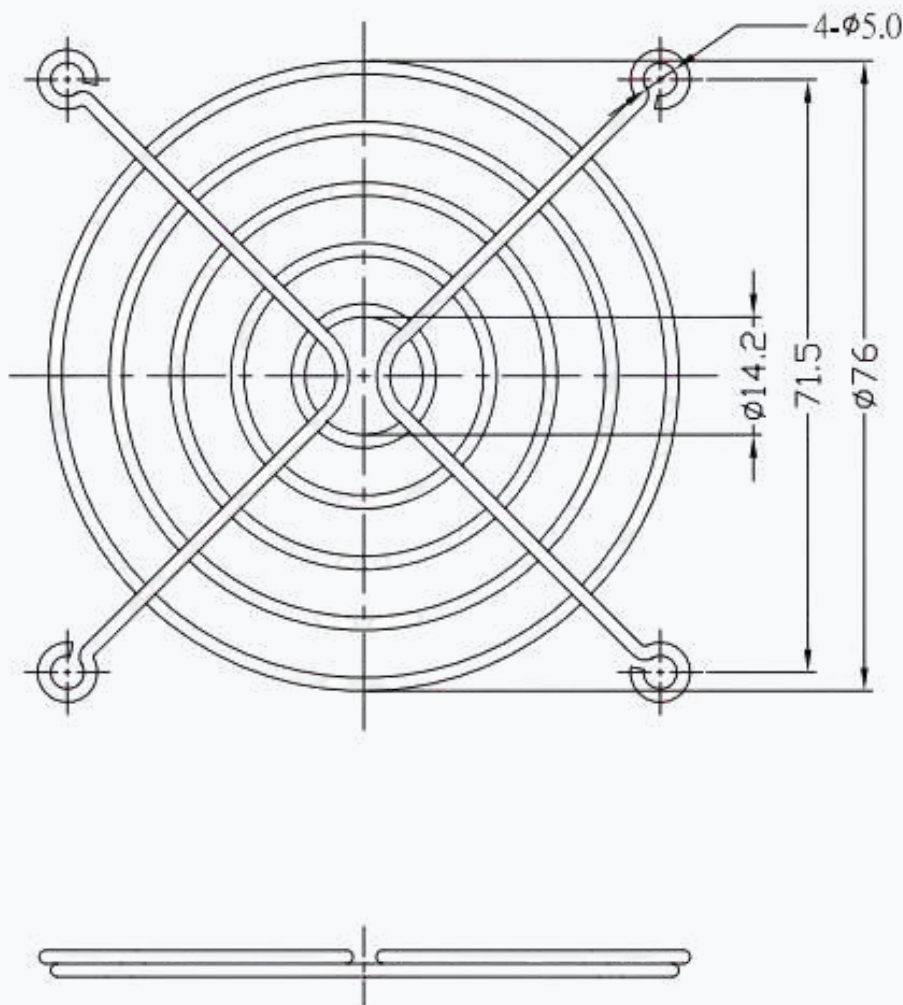
Dimensions (mm)
