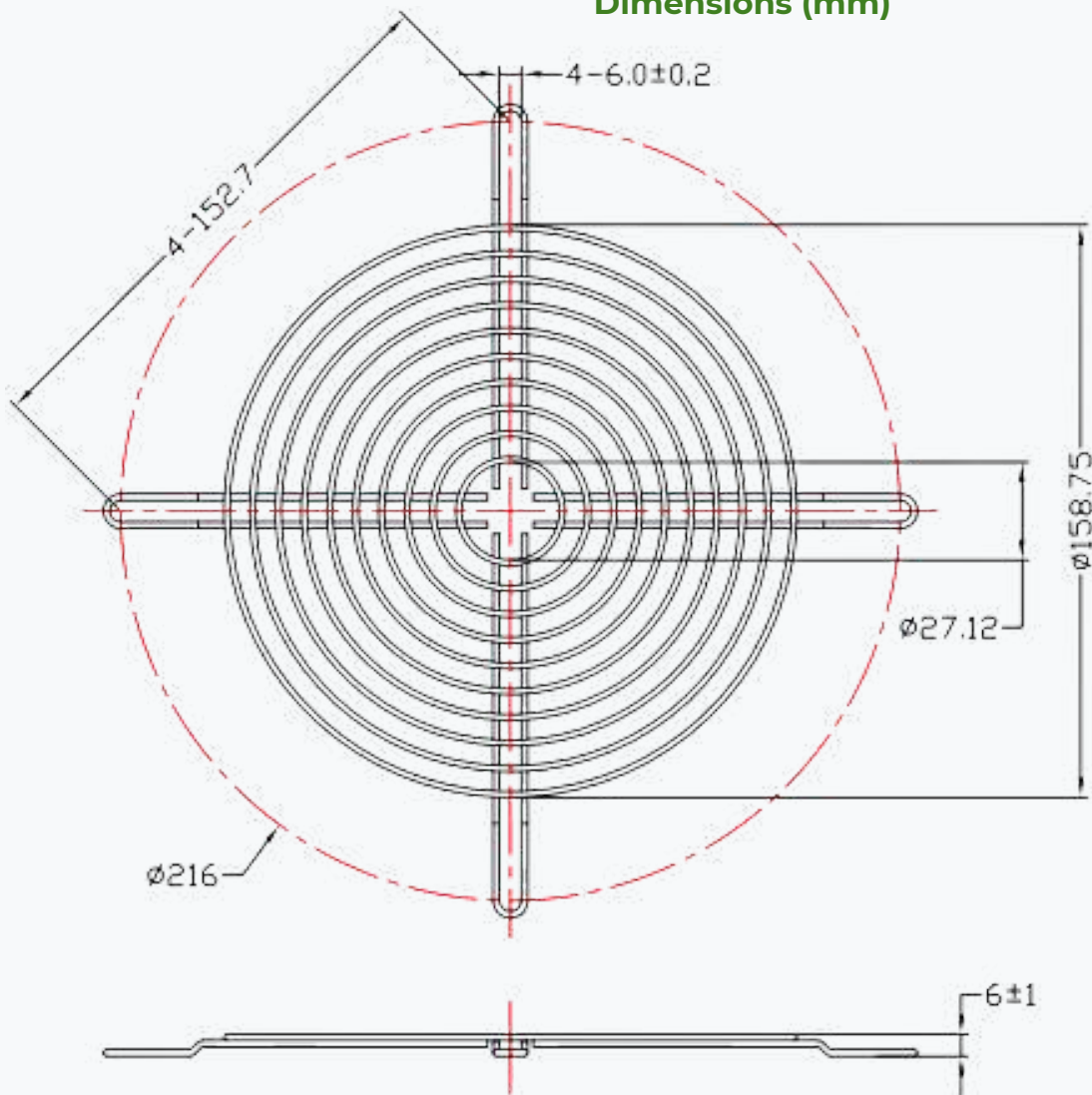
Dimensions (mm)
