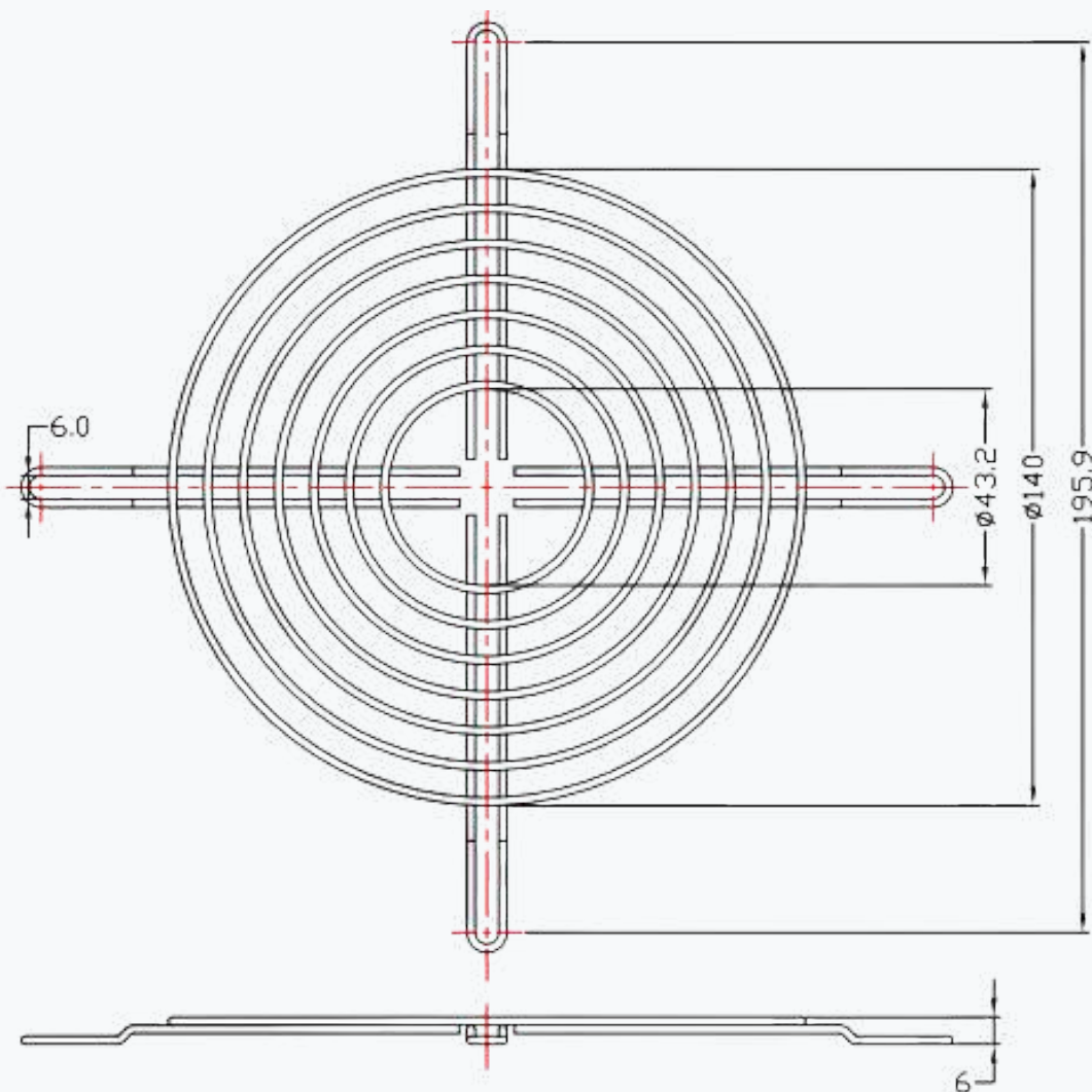
Dimensions (mm)
