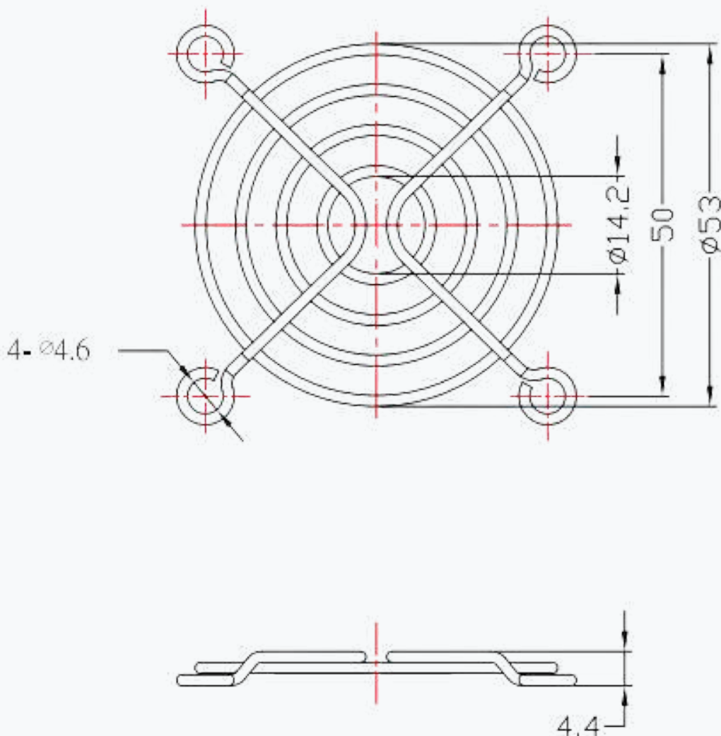
Dimensions (mm)
