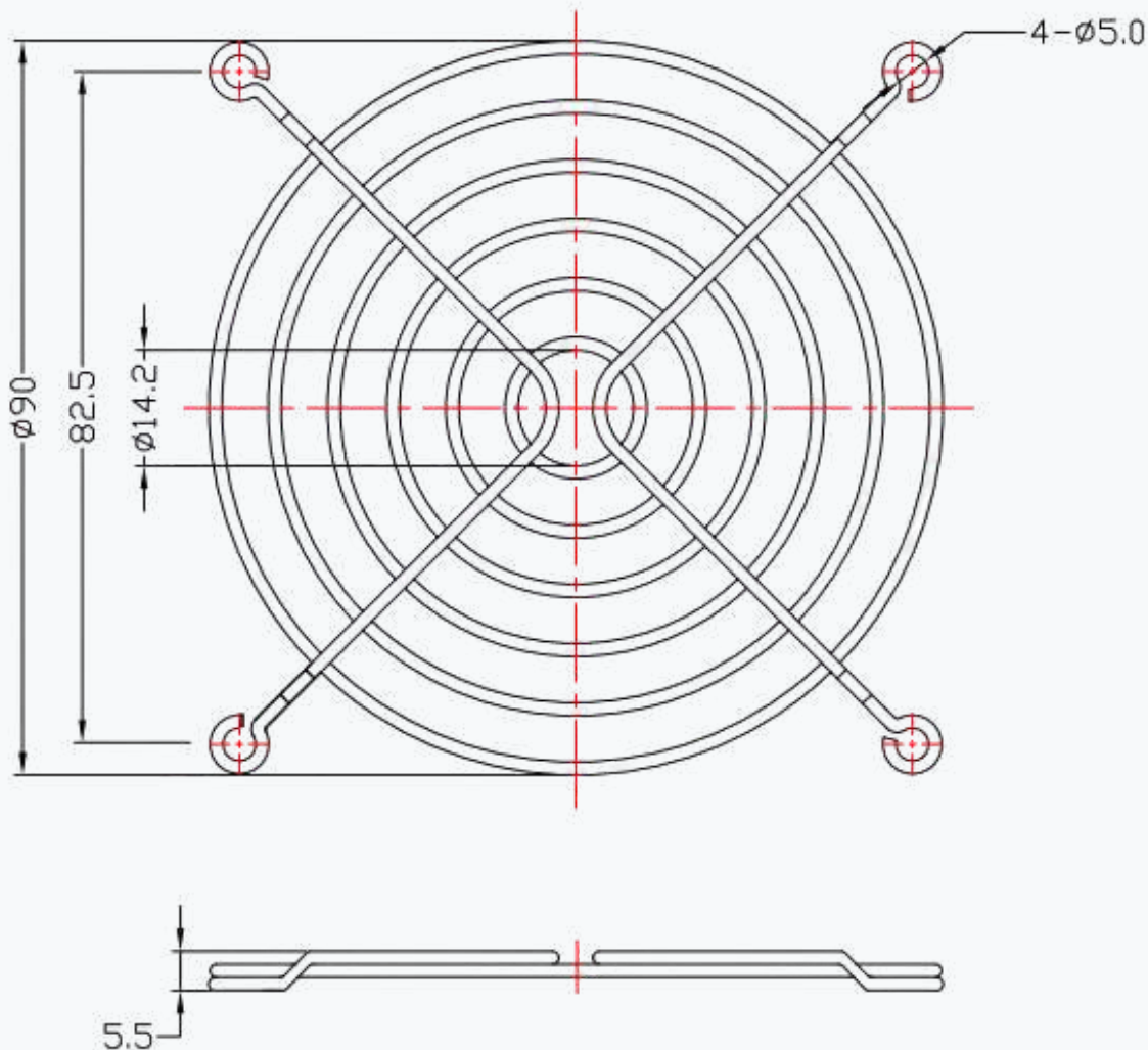
Dimensions (mm)
