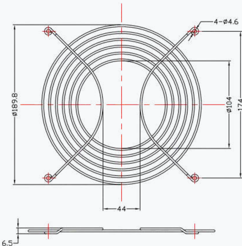
Dimensions (mm)
