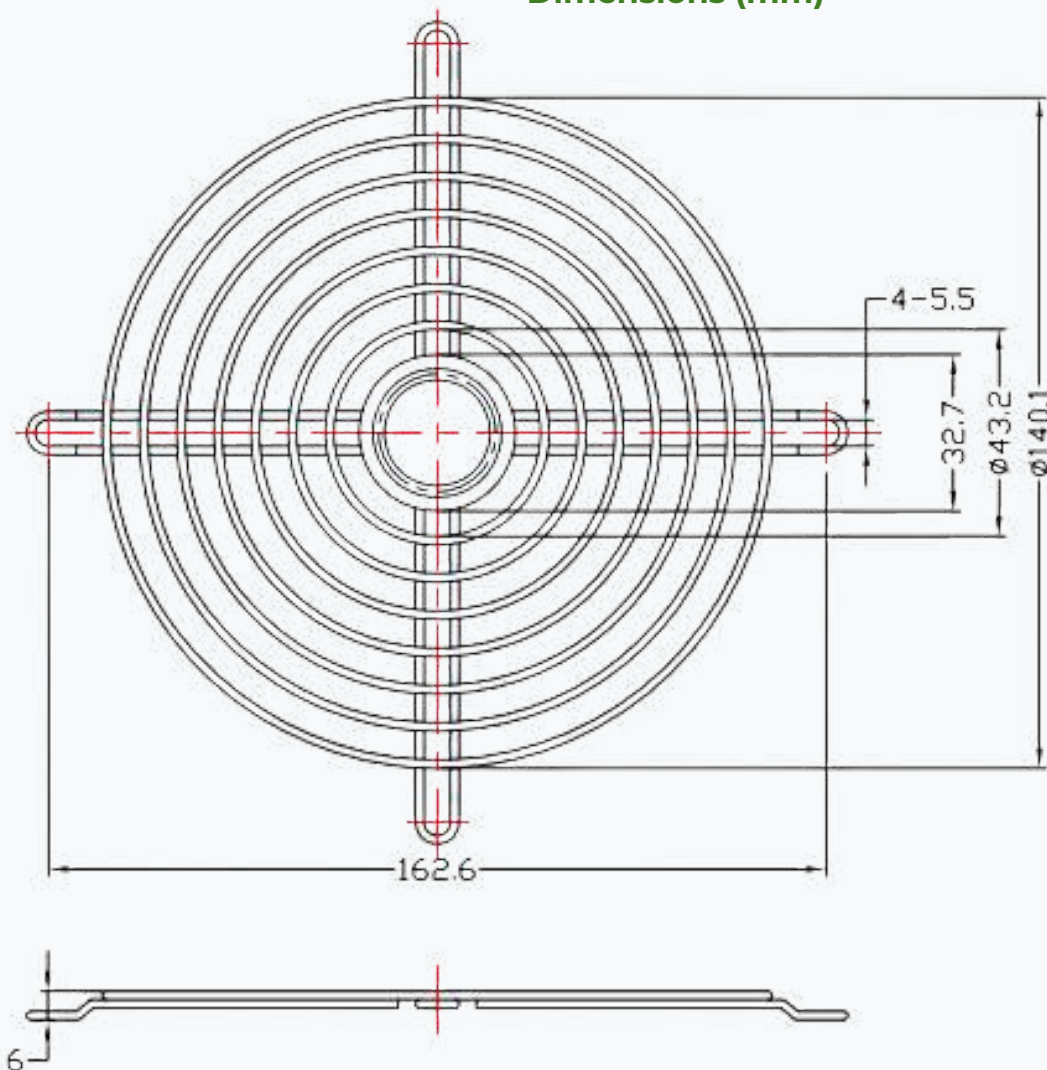
Dimensions (mm)
